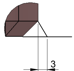
Welding detail
