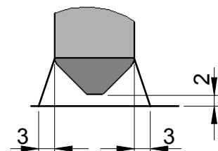
Welding detail
