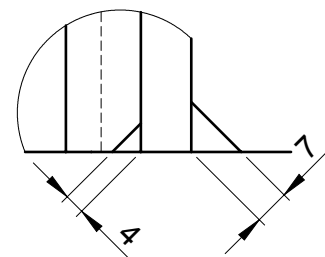
Welding detail
