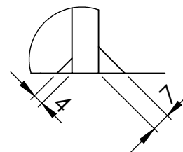
Welding detail
